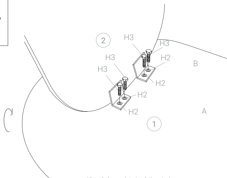
Vista de la cara interior de la pata / View of the inner side of the leg
