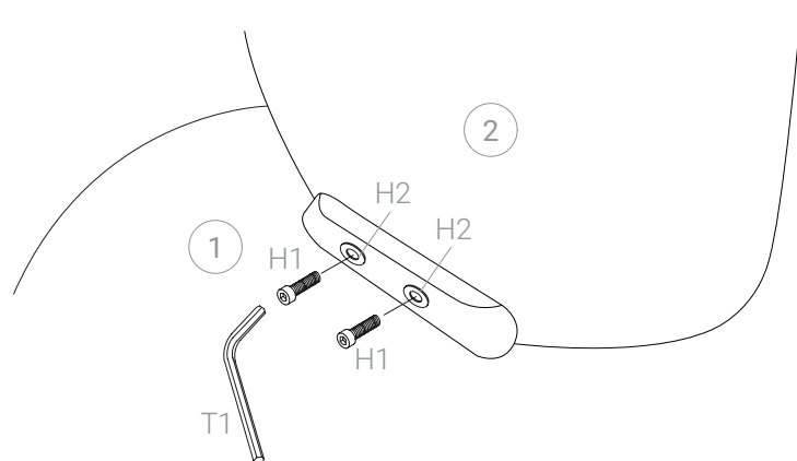
Vista de la cara exterior de la pata / View of the outer side of the leg
