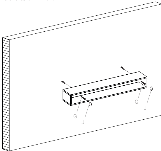
PASO 3.5/STEP 3.5
